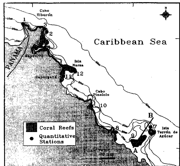
FIG. 2. - Northwestern part of the Golfo de Urabá showing the distribution of hard bottoms with coral cover and the location of sampling stations. Straight line A-B marks the location of the schematic profile of Figure 7.
