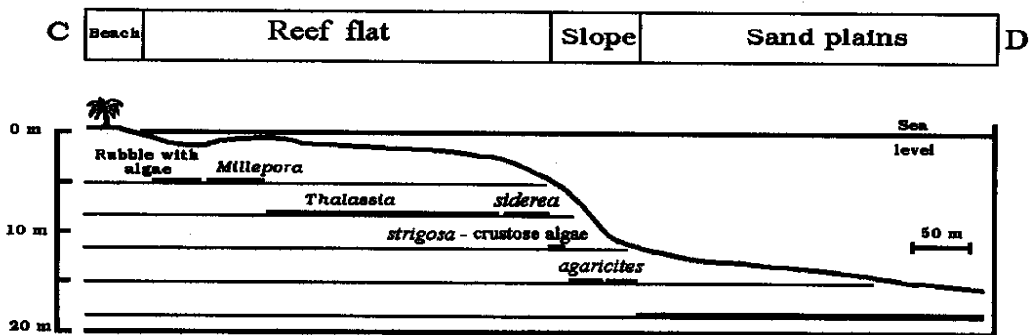
FIG. 6. – Schematic profile (straight line C-D in Fig. 5) showing the zonation of coral assemblages and bottom type habitats in the bay of Capurganá.
