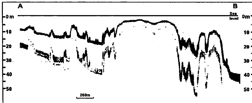
FIG. 7. – Echosounder bathymetric profile across the mid relief spurs between the mainland coast and the islet Terrón de Azúcar (straight line A-B in Fig. 2). The upper parts of the high reliefs in the left half of the profile are covered by the 'Agaricia spp.' assemblage, the deeper ones by the 'mixed corals' assemblage.
