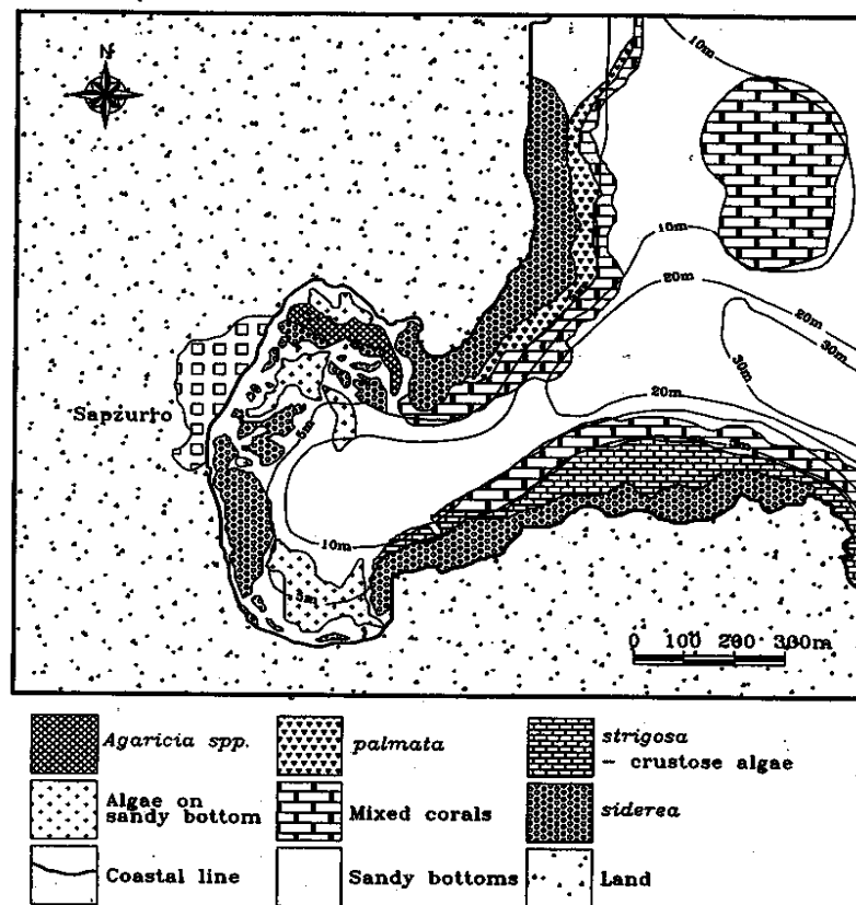
FIG. 4. - Bottom topography and distribution of coral assemblages and other bottom habitats within and off the Cove of Sapzurro.
